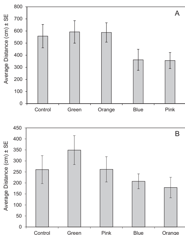
Fig. 3. Outcomes of laboratory experiments investigating the vertical distance (cm \pm SE) climbed by (A) adult and (B) nymph Halyomorpha halys marked with four different colors of fluorescent powder and an unmarked control (no statistical differences among treatments; A: ANOVA, P = 0.245 and B: ANOVA, P = 0.317 ).
